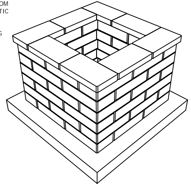
ISOMETRIC VIEW
