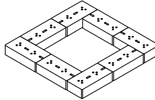
ISOMETRIC VIEW
