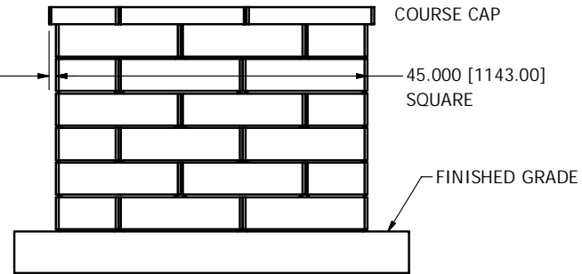
SIDE ELEVATION VIEW
